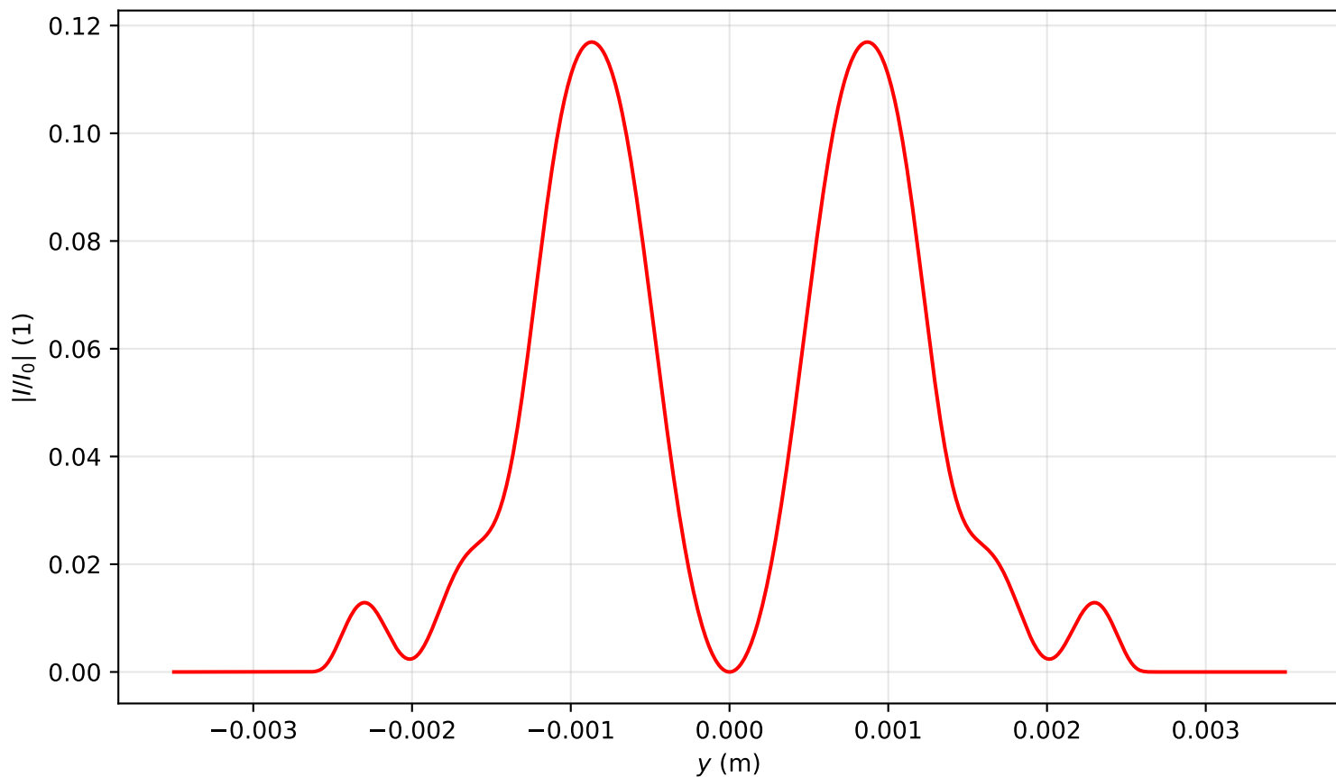
Intensity profile I(x=0, y, z=3.582)/I_0 , \text{Pin}=4.0\text{Pcr} , artificial time
